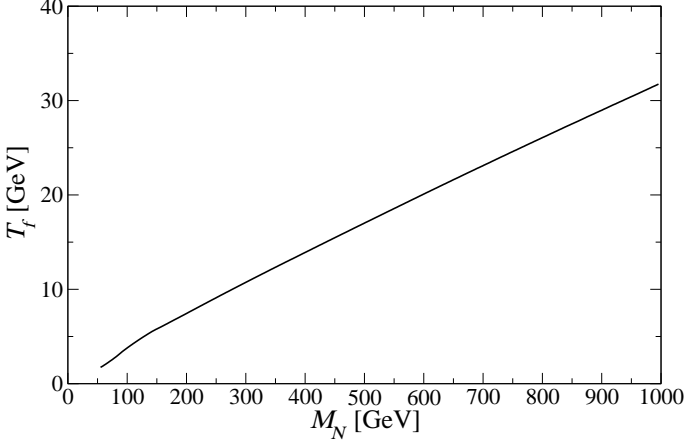
Fig. 2. The freeze-out temperature (in \text{GeV} \approx 1.16 \times 10^{13} \text{ K} ) of heavy neutrinos as a function of their mass (in \text{GeV} ).
