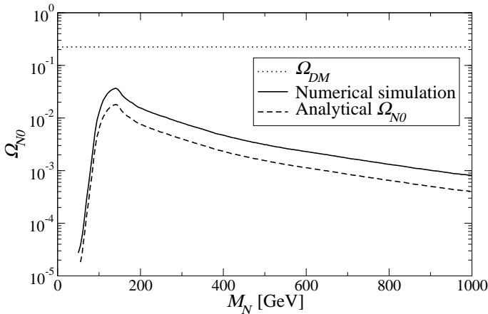
Fig. 3. The relic relative density of heavy neutrinos as a function of their mass (in \text{GeV} ).
