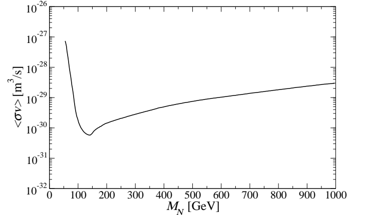
Fig. 1. The cross section times the velocity (in m^3/s ) of heavy neutrino annihilation N\bar{N} as a function of their mass (in GeV) at freeze-out, T = T_f .
